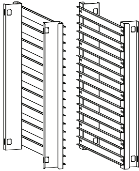
1/2 Height 1-piece Construction Part No: C5-13-L5
