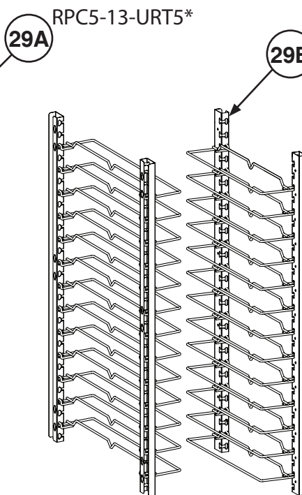
3/4 Height RPC5-13-U7 (includes slides and uprights)
