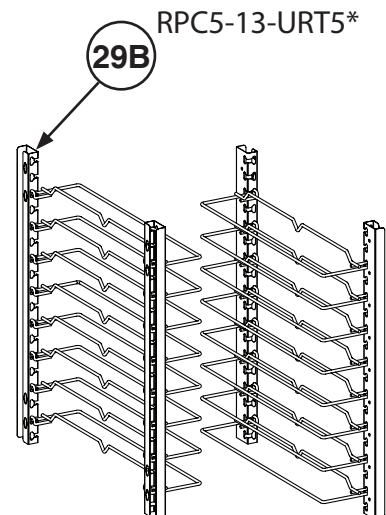
1/2 Height RPC5-13-U5 (includes slides and uprights)
